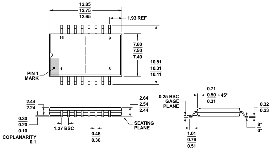
COMPLIANT TO JEDEC STANDARDS MS-013-AC Figure 19. 16-Lead Standard Small Outline Package, with Increased Creepage [SOIC_IC] Wide Body (RI-16-2) Dimensions shown in millimeters
